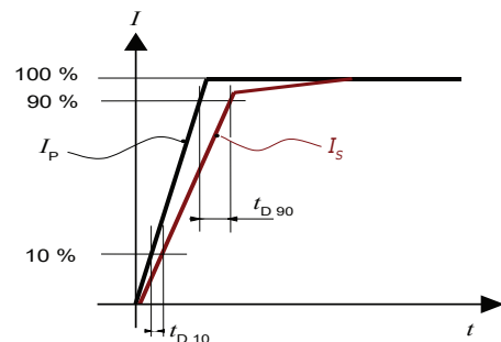
Figure 26: t_{D10} (delay time to 10 %) and t_{D90} (delay time to 90 %)
