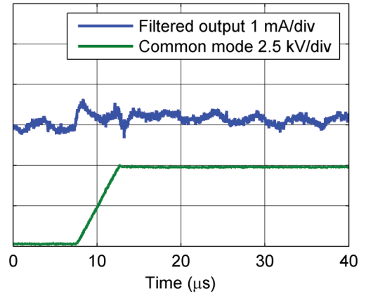
Figure 19: Typical common mode perturbation with 10 kHz 1 st order low pass filter on the output (5 kV step with 1 kV/ \mu s, R_M = 1 \Omega )
