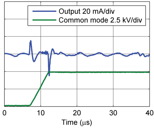
Figure 18: Typical common mode perturbation, unfiltered output (5 kV step with 1 kV/ \mu s, R_M = 1 \Omega )
